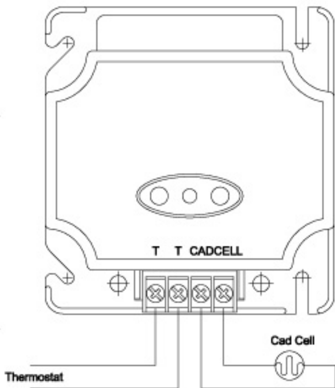
Wiring Diagram
